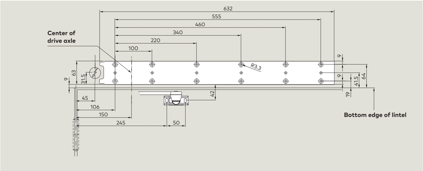
Drilling template: BASIC cover, push-version, standard axle extension
