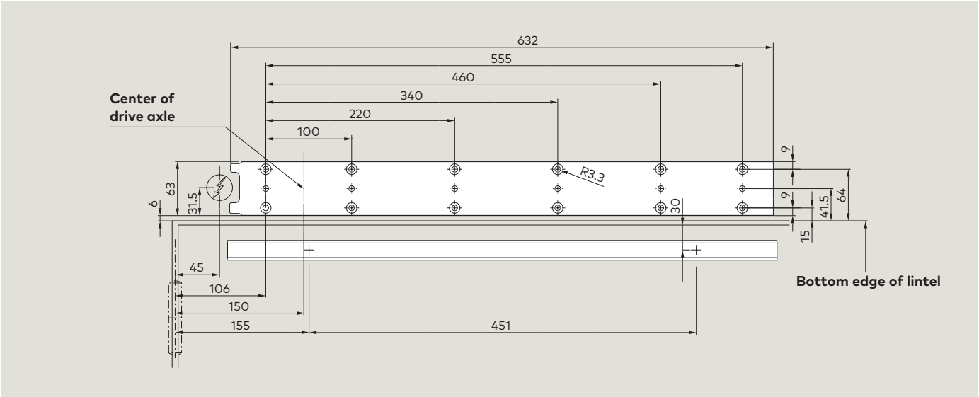
Drilling template: BASIC cover, push-version, 12.5 mm pivot pin, standard axle extension
