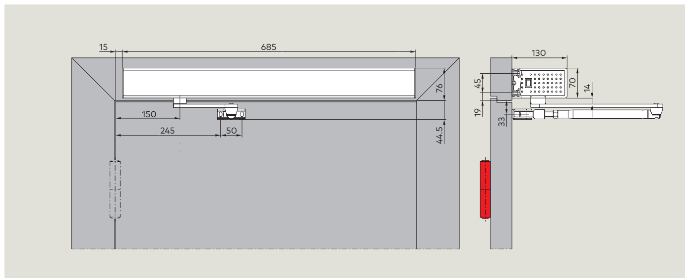
View: BASIC cover, push-version, standard axle extension
