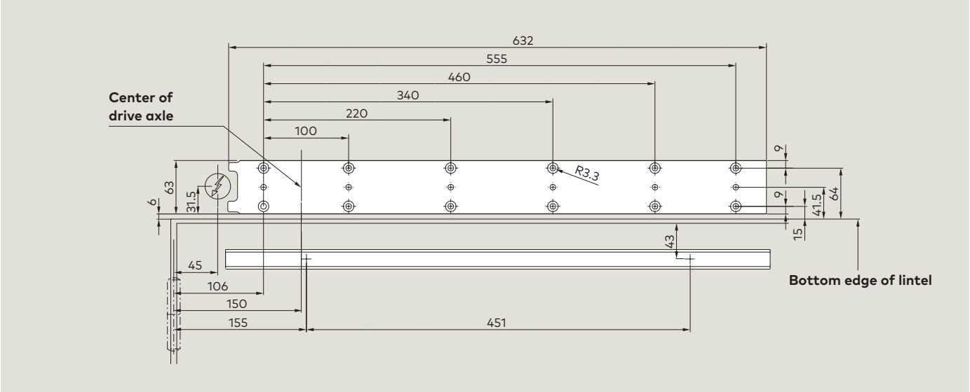
Drilling template: BASIC cover, push-version, 25 mm pivot pin, standard axle extension
