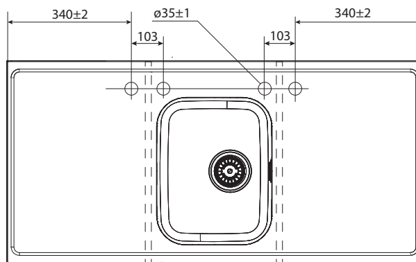
Sink unit 1200
