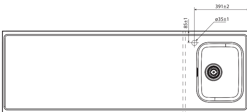
Sink unit 800 1000 1200 1800
