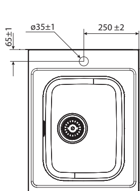
Sink unit 500
